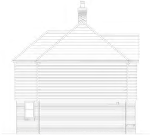
PLOT 55 SIDE ELEVATION
